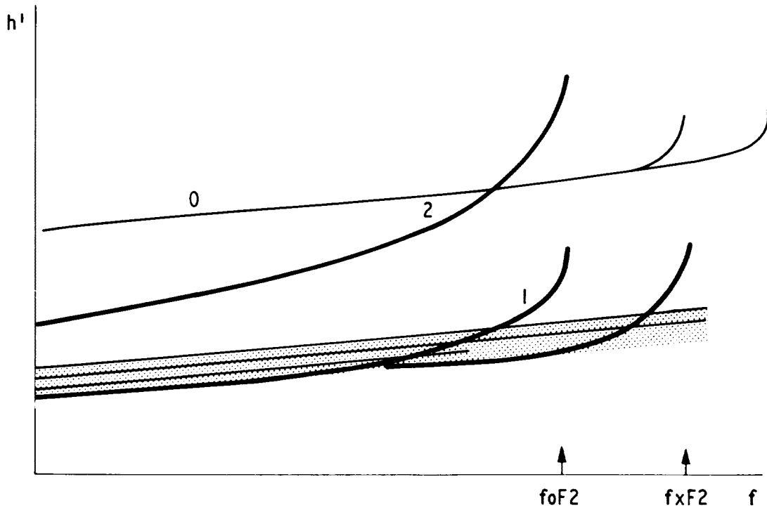
Fig. 2.15 Range spreading
