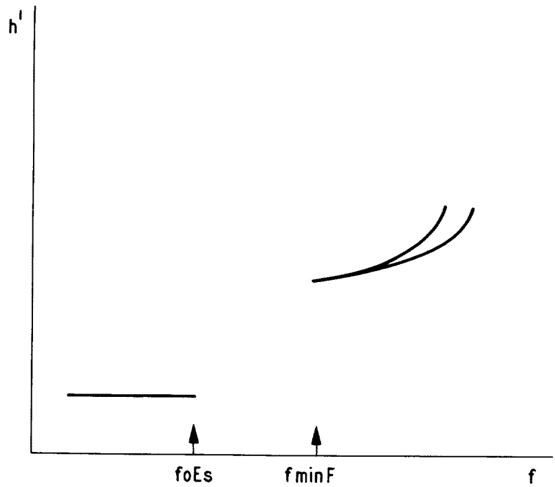
Fig. 4.22 Trace missing due to a severely tilted layer f_b E_s = Y unless accuracy rules allow an estimated value to be made. If in doubt use Y .
