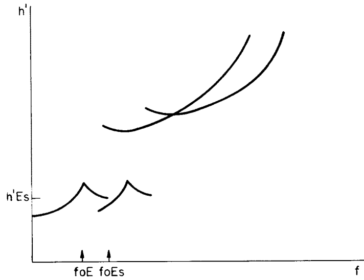
Fig. 3.18 Use of G with h'Es h'Es = (h'Es)EG
