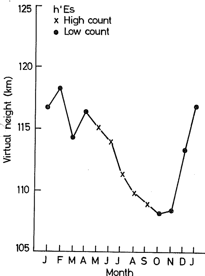
Seasonal variation of the mean value of h'Es for Slough. Six year data have been averaged.
