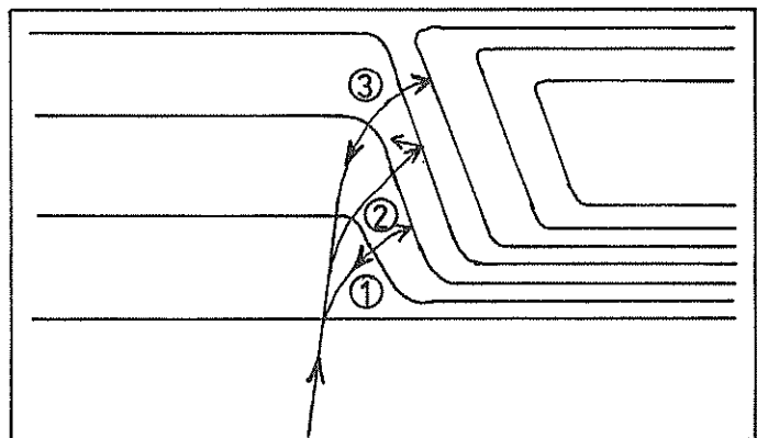
Figure 1. Possible iso-ionic contours and ray paths for three frequencies, 1. 4.5MHz, 2. 6.5MHz and 3. 7.5MHz
