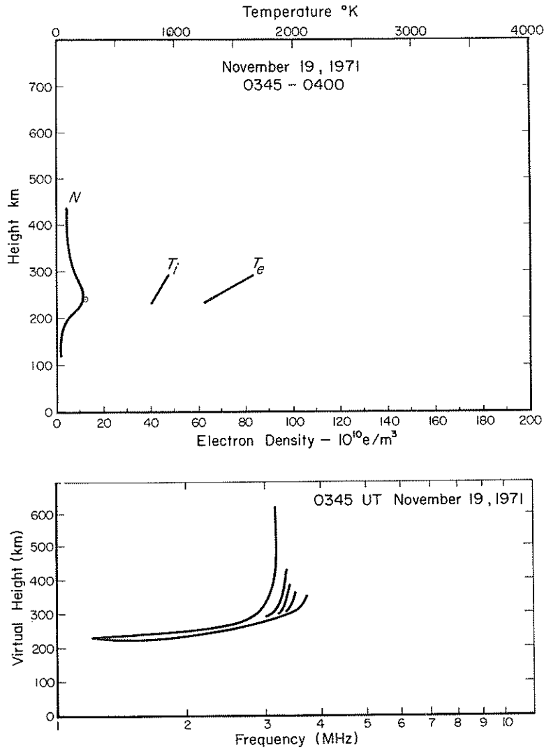
Figure 10. Simultaneous College ionogram showing spread F and Chatanika N(h) for November 19, 1971, 0345 UT, 1745 LMT.
