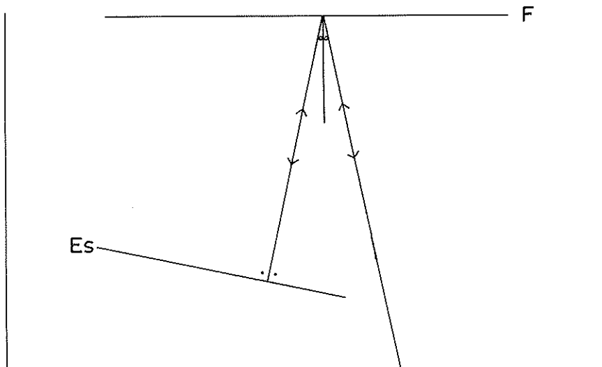
Figure 2. Mode of reflection from a horizontal F layer and tilted Es or E layer (oblique M reflection).
