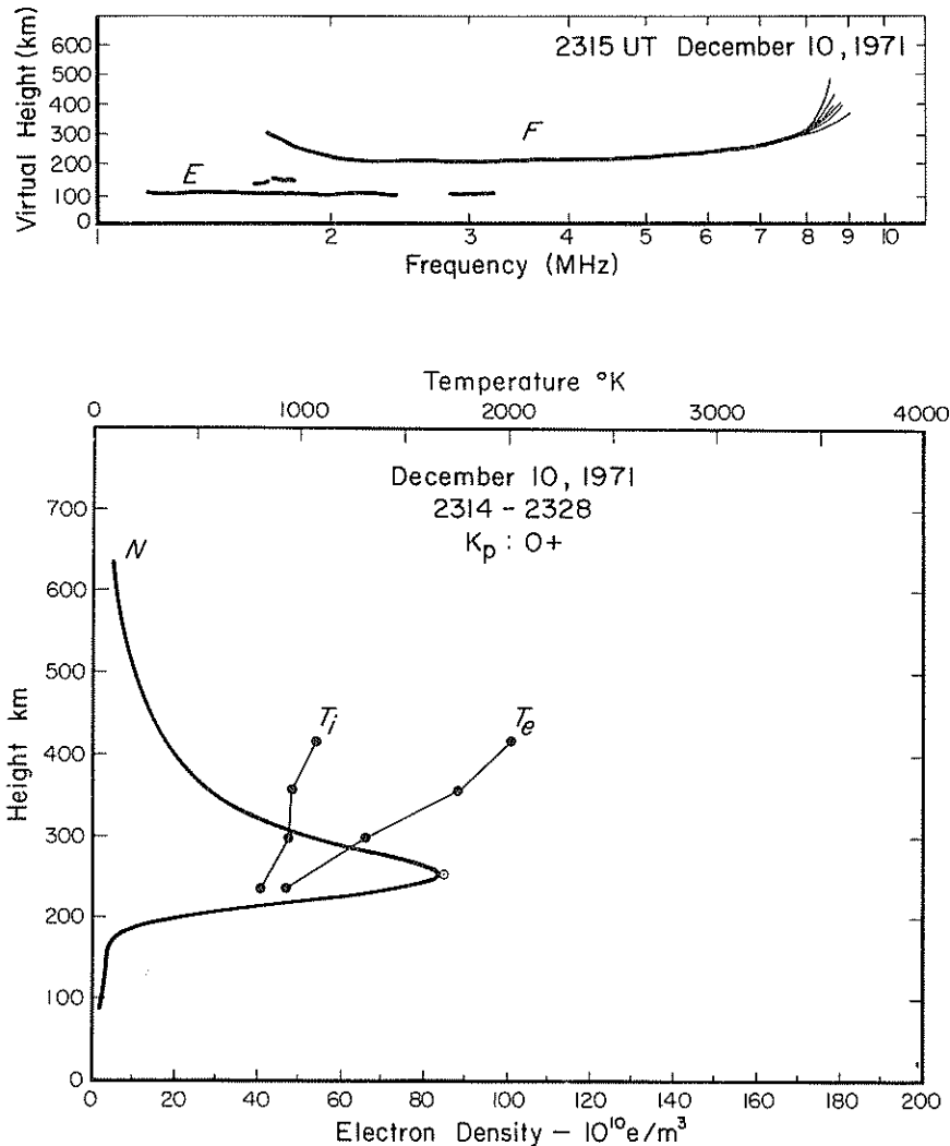
Figure 5. Simultaneous College ionogram and Chatanika radar N(h) for December 10, 1971, 2315 UT, 1315 LMT.
