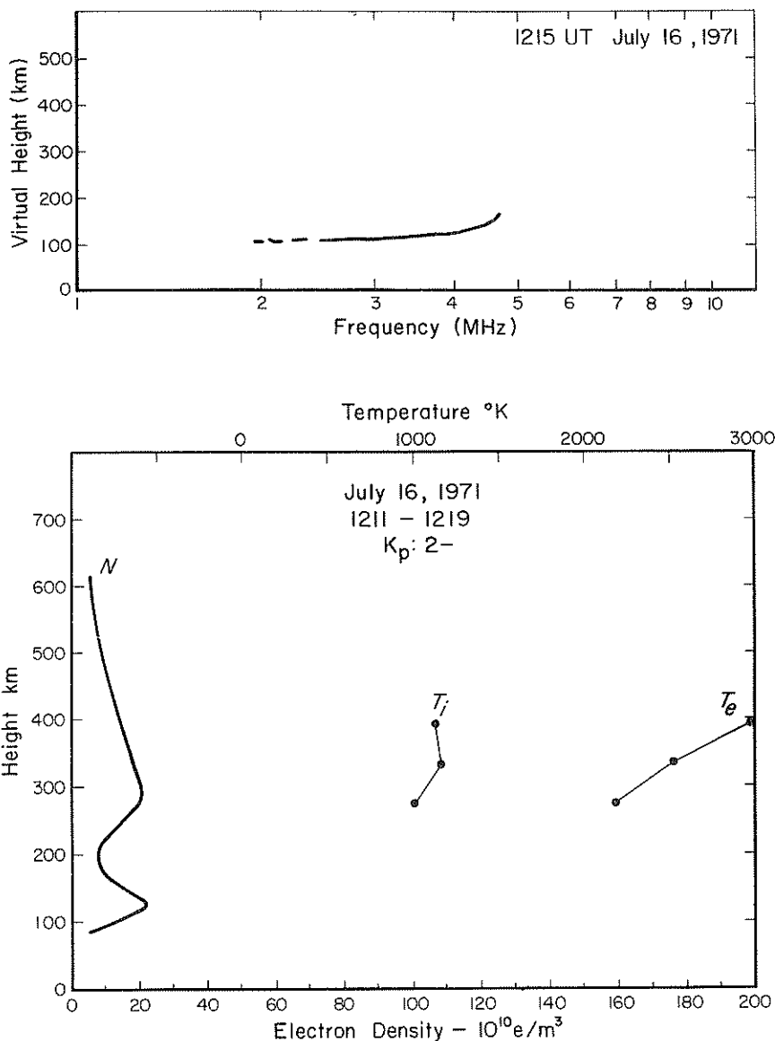
Figure 3. Simultaneous College ionogram and Chatanika radar N(h) for July 16, 1971, 1215 UT, 0215 LMT.
